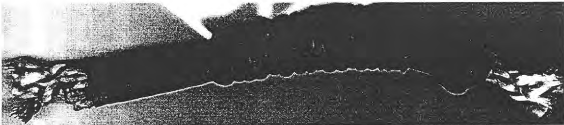
Figure 7: Accordion-type deformation typically observed in the deformation stages following the peak load. This sample is from TEST 7 and is shown at 75% of actual size.
